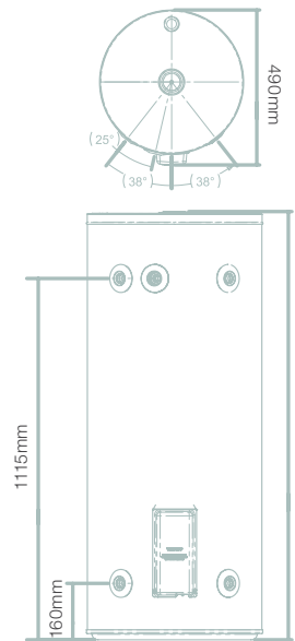
125L NARROW DIAMETER SPECIFICATIONS
